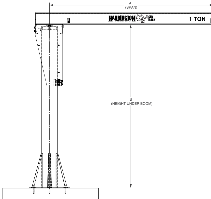
Foundation Mounted
